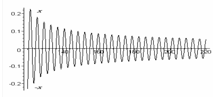
Fig.5. Particle oscillation in well and its gradual disappearance (“crematorim” solution).
