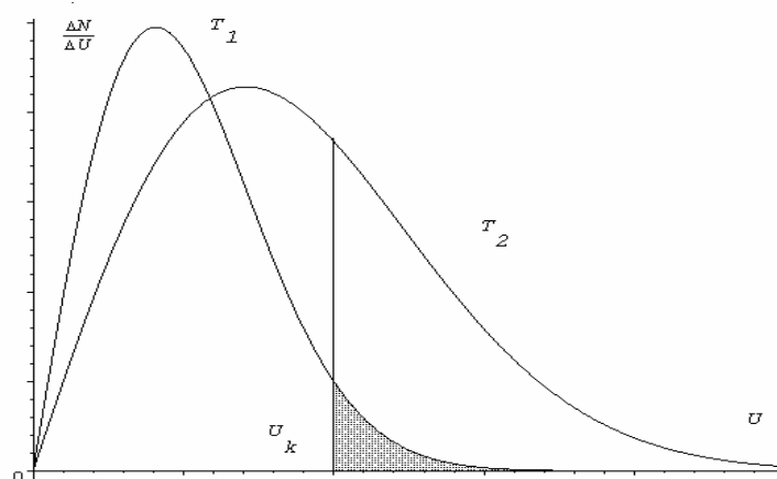
Fig.8. Distribution of molecules by kinetic energy ( T_1 < T_2 ).
