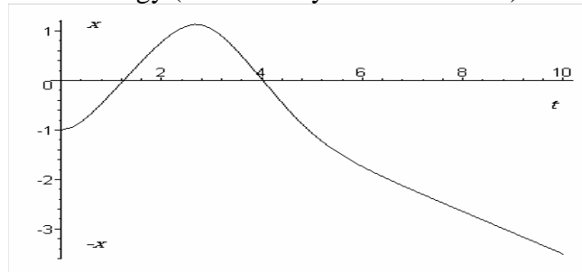
Fig.1. Reflection from potential well with a certain speed increase.
