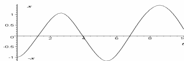
Fig.3. Oscillation in well with energy growth ("maternity home" solution).
