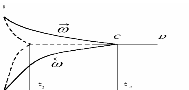
Fig. 10. Establishment of chemical equilibrium. Along axis x-time, along axis y- reaction speed. Firm line – without catalyst, dotted line – with catalyst. CD – chemical equilibrium line; t_1 \ll t_2 .
