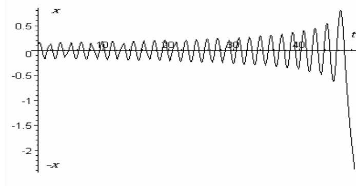
Fig.4. Passage of well with oscillations and energy growth (“Mathernity Home” solution).
