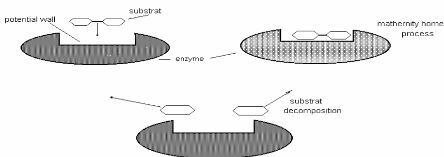
Fig.7. Disintegration of polysaccharides molecule in presence of lysozyme
