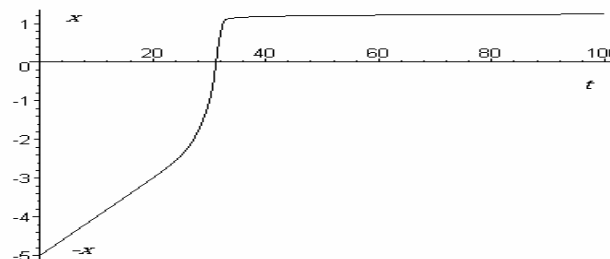
Fig.6. Passage of well with nearly full loss of energy.
