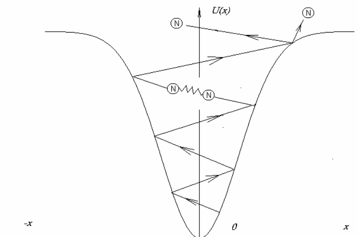
Fig.12. Oscillation of Nitrogen molecule in potential well of catalyst.
