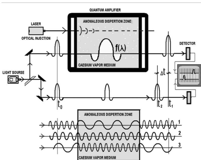
Figure 5. Experiments of L. Wang - superluminal light propagation
