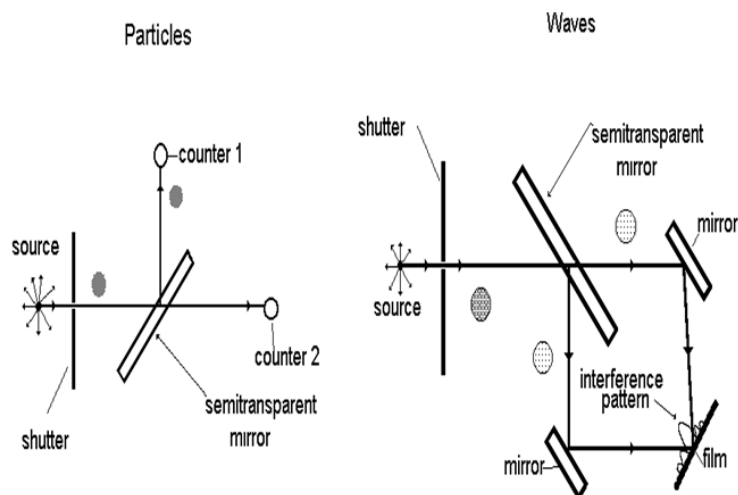
Figure 1. Experiments with individual photons on semitransparent mirror
