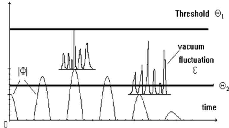
Figure 4. Quantum measurements
